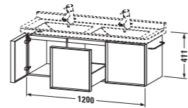
# 6107 ↔ 1200 mm, ↗ 479 (435) mm → Starck 3 # 0332130000, 1300 mm
