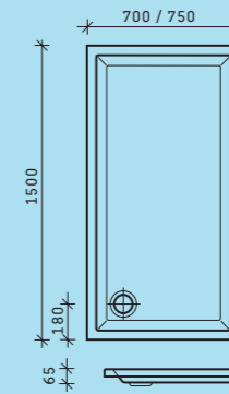
# 720036 1500 x 700 mm # 720037 1500 x 750 mm
