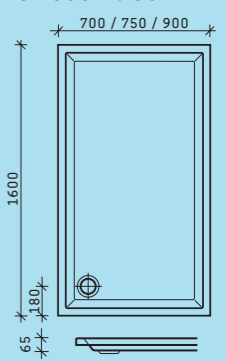
# 720038 1600 x 700 mm # 720039 1600 x 750 mm # 720040 1600 x 900 mm
